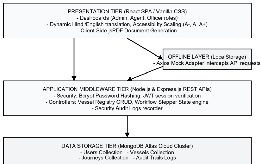
Figure 3.1: High-Level System Architecture Diagram
