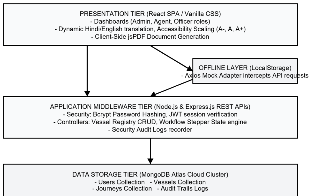
Figure 1.1: High-Level System Architecture Overview
